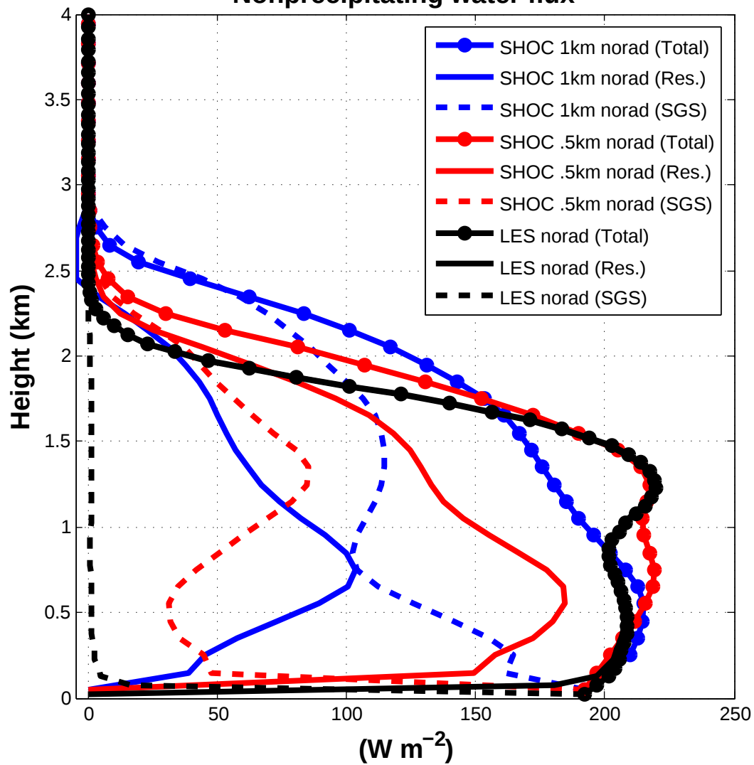
Nonprecipitating water flux
