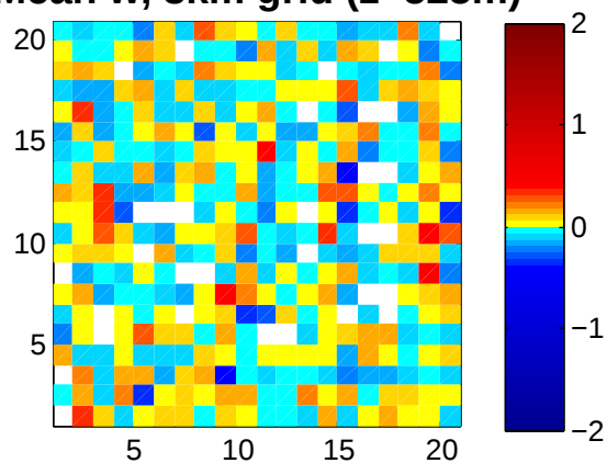
Mean w, 3km grid (z=525m)
