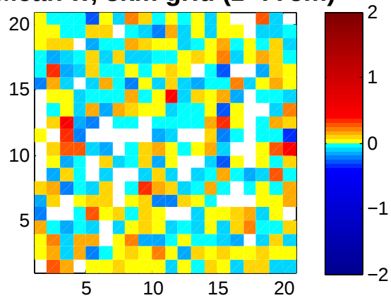
Mean w, 3km grid (z=775m)
