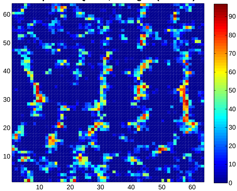
% of pts with QN > 0, 1km grid (z=775m)
