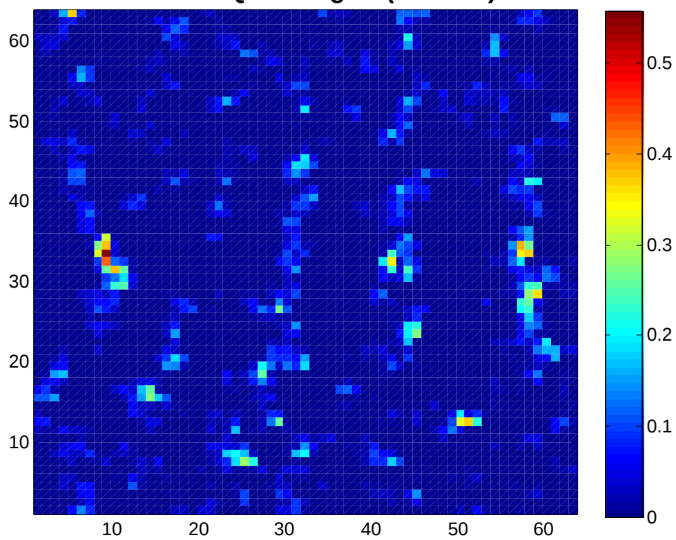
RMSE of QP 1km grid (z=775m)
