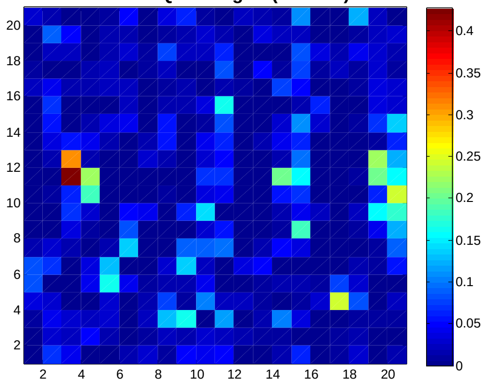
RMSE of QP 3km grid (z=775m)
