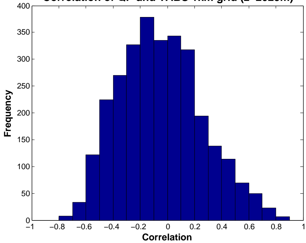
Correlation of QP and TABS 1km grid (z=2025m)
