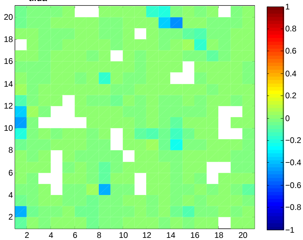
TI tilda – TI (25th percentile), 3km grid (z=2025m)
