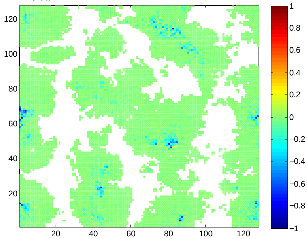
TI_{\text{tilda}} - TI (25th percentile), .5km grid (z=2025m)
