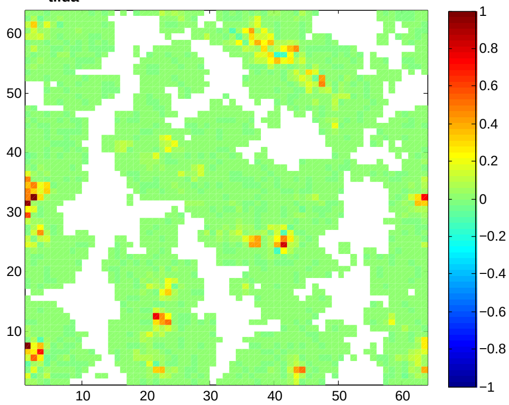
TI_{\text{tilda}} - TI (75th percentile), 1km grid (z=2025m)
