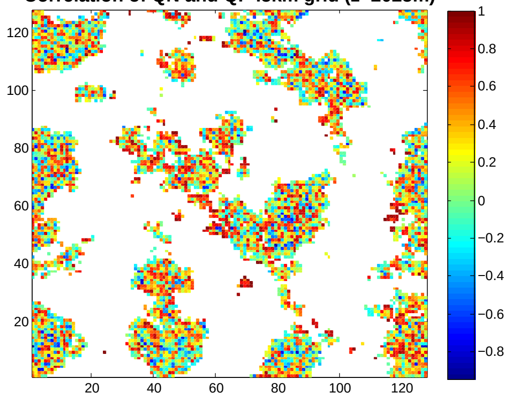
Correlation of QN and QP .5km grid (z=2025m)
