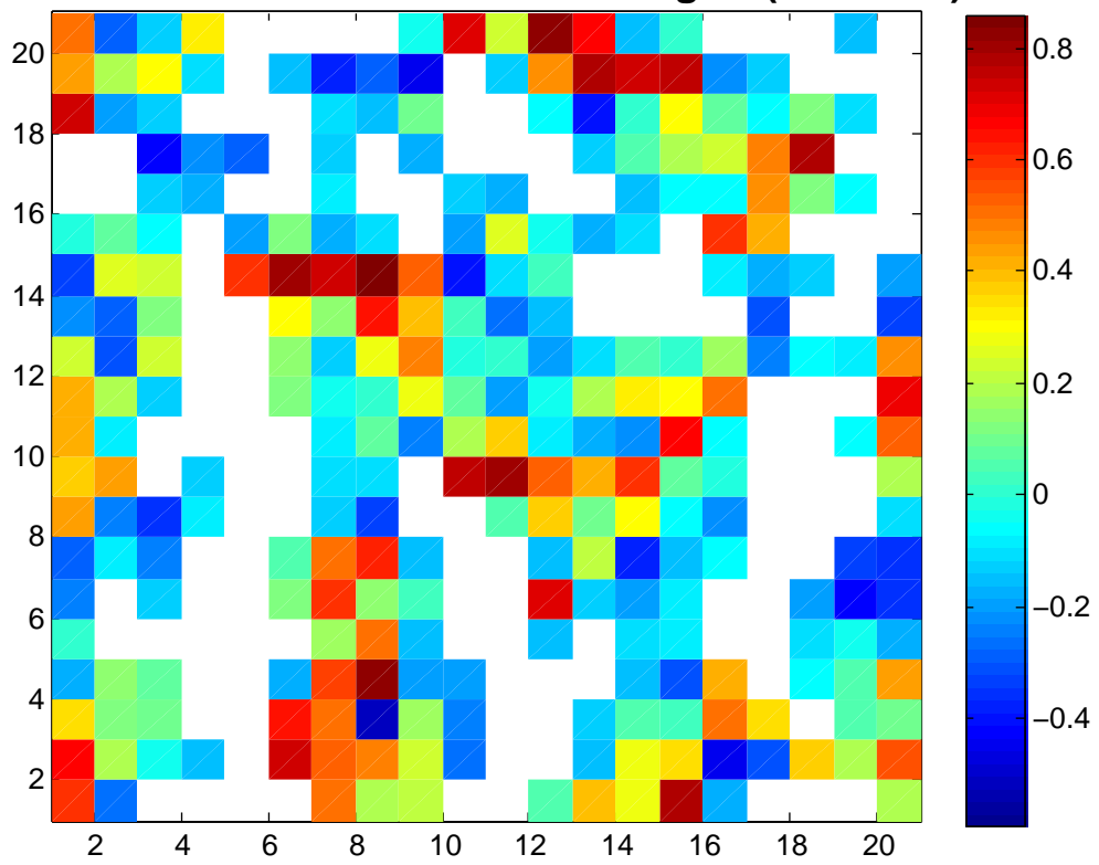
Correlation of QN and TABS 3km grid (z=2025m)
