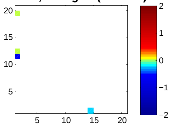
Mean w, 3km grid (z=525m)
