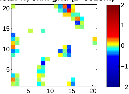
Mean w, 3km grid (z=3025m)
