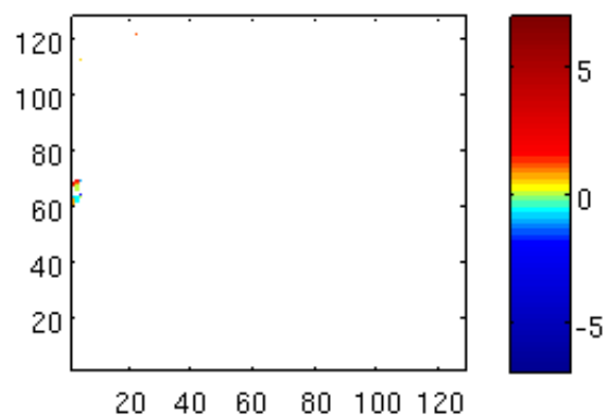
Mean w, .5km grid (z=525m)
