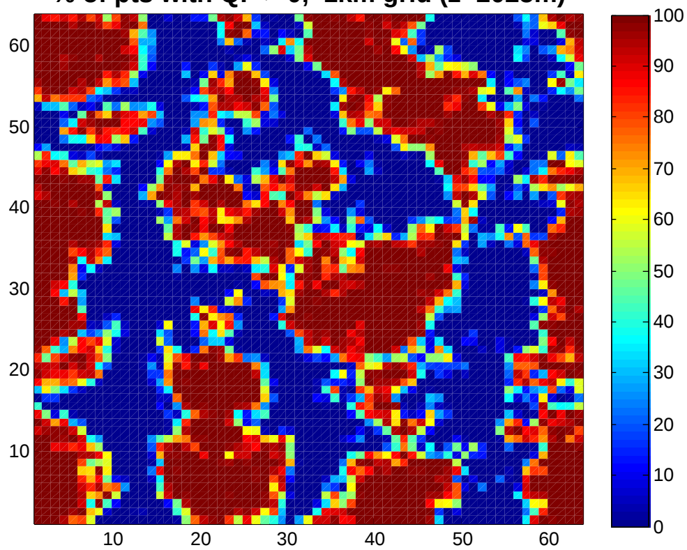
% of pts with QP > 0, 1km grid (z=2025m)
