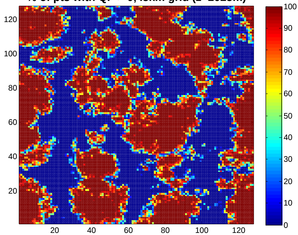
% of pts with QP > 0, .5km grid (z=2025m)
