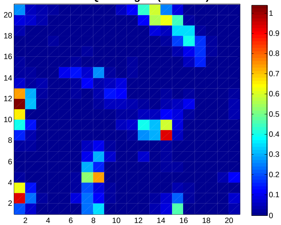
RMSE of QP 3km grid (z=2025m)
