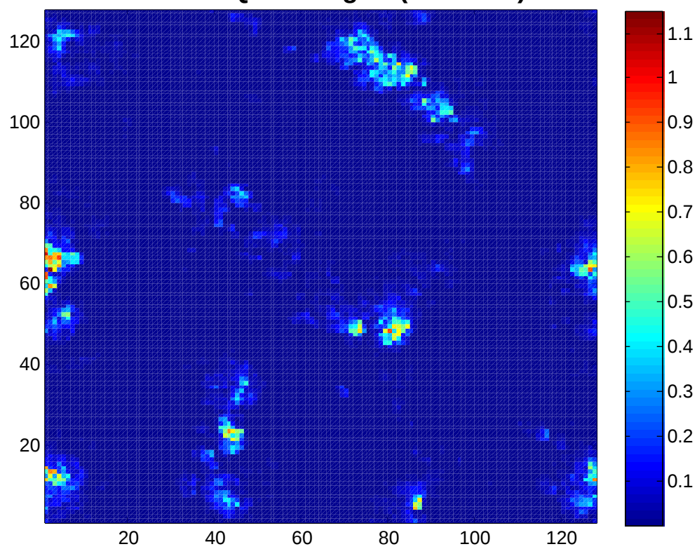
RMSE of QP .5km grid (z=2025m)
