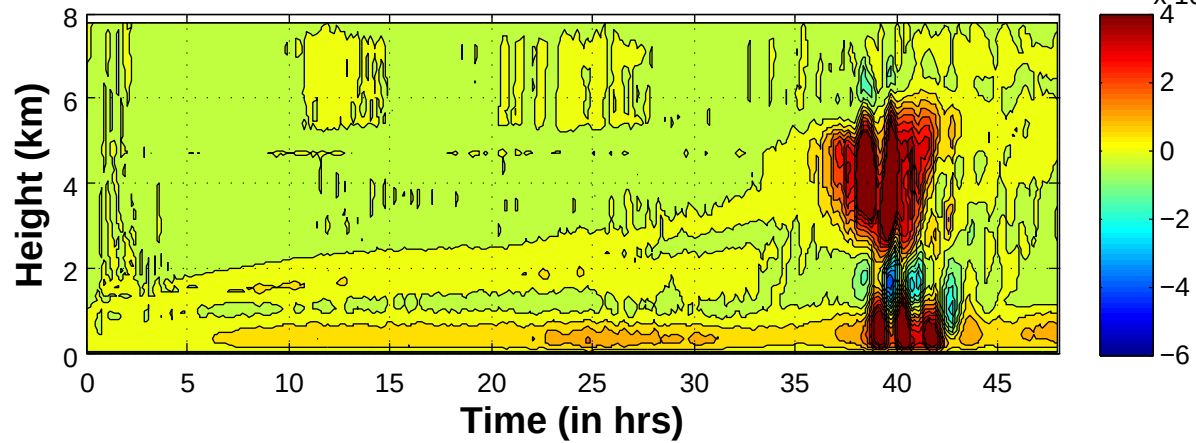
SGS Buoyancy production terms of TKE ( \text{W m}^{-2} \text{sfc-flx-fxd-T-v2} ) \times 10^{-3}
