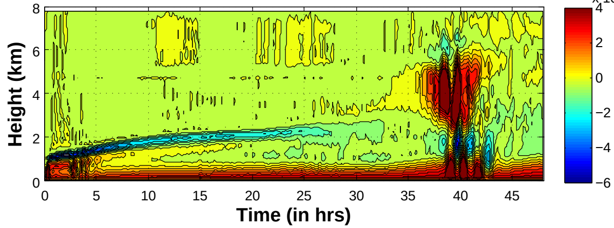
Resolved Buoyancy production terms of TKE ( \text{W m}^{-2} \text{sfc-flx-fxd-T-v2} ) \times 10^{-3}
