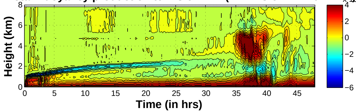
Resolved Buoyancy production terms of TKE ( \text{W m}^{-2} \text{sfc-flx-fxd-T-v2} ) \times 10^{-3}
