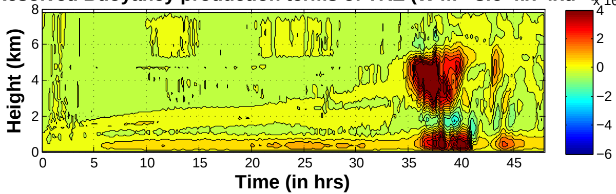
SGS Buoyancy production terms of TKE ( \text{W m}^{-2} \text{sfc-flx-fxd-T-v2} ) \times 10^{-3}
