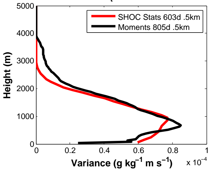
Total \langle W'Q'_t \rangle .5km Ice Only
