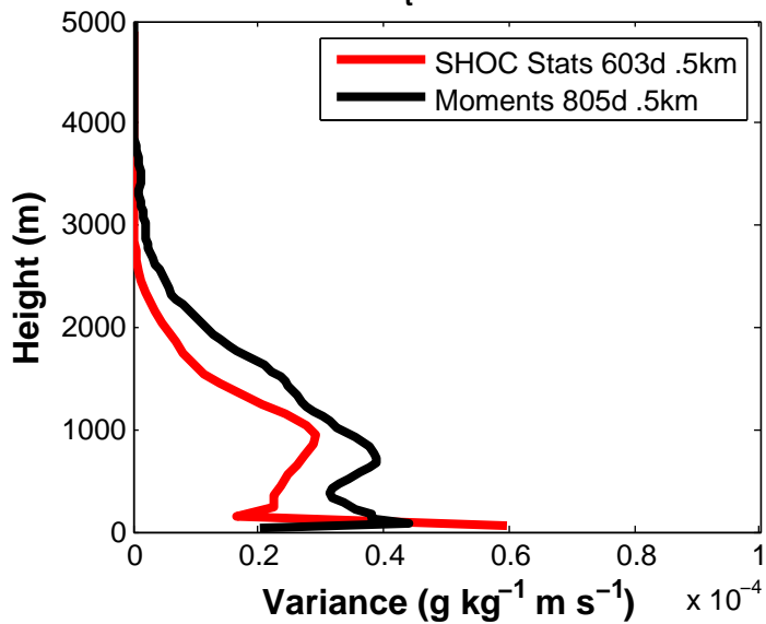
SGS \langle W'Q'_t \rangle .5km Ice Only
