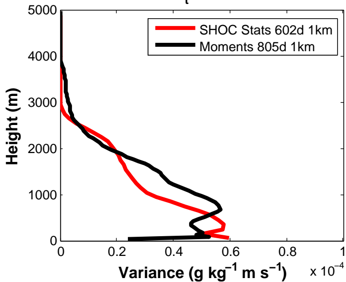
SGS \langle W'Q'_t \rangle 1km Ice Only
