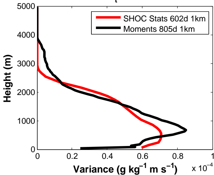
Total \langle W'Q'_t \rangle 1km Ice Only
