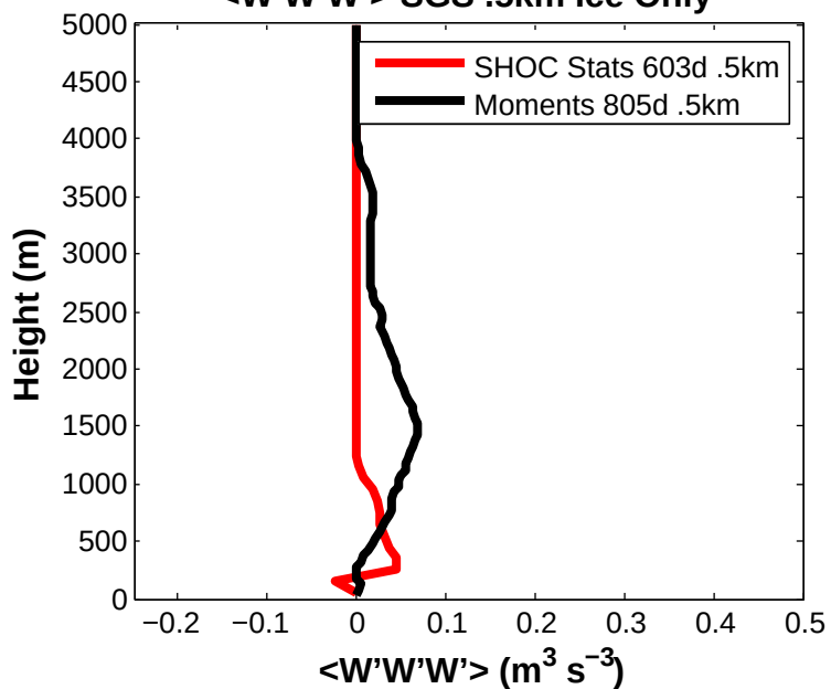
<W'W'W'> SGS .5km Ice Only
