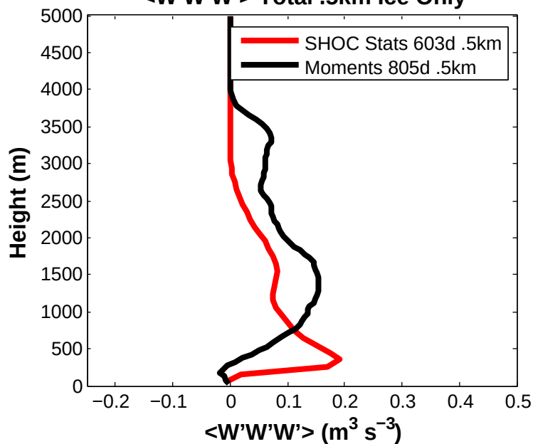
<W'W'W'> Total .5km Ice Only
