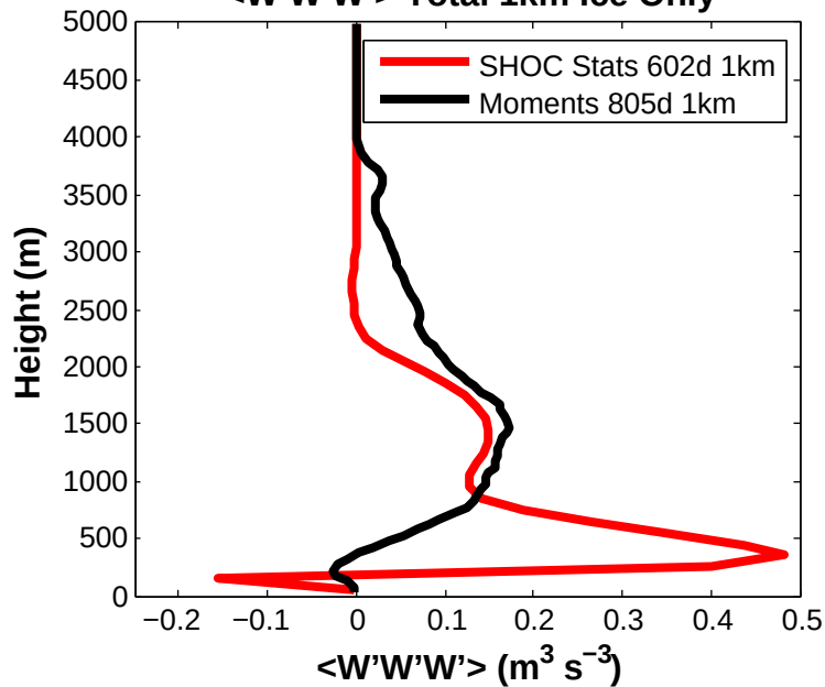
<W'W'W'> Total 1km Ice Only
