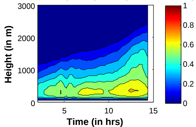
Total \langle W'W' \rangle ( \text{m}^2 \text{s}^{-2} ) 603d (SHOC ice .5km)
