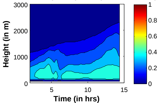
SGS \langle W'W' \rangle ( \text{m}^2 \text{s}^{-2} ) 603d (SHOC ice .5km)
