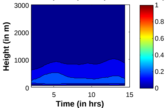
SGS \langle W'W' \rangle ( \text{m}^2 \text{s}^{-2} ) 805d (LES ice)
