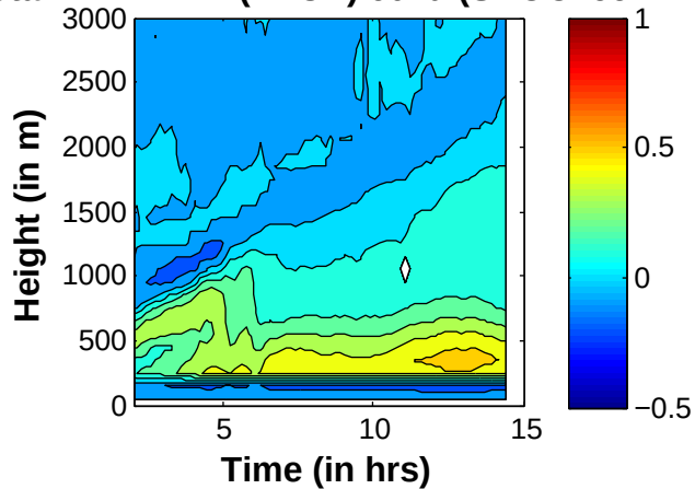
Total \langle W'W'W' \rangle ( \text{m}^2 \text{s}^{-2} ) 603d (SHOC ice .5km)
