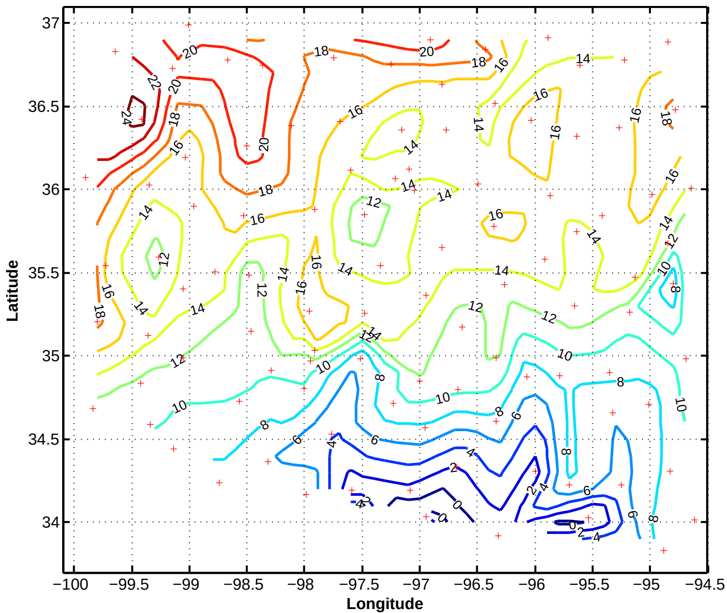
6/14/97 0000z Mesonet Pressure in .1mb above 970mb
