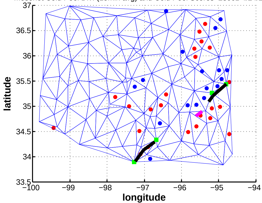
Mesonet Cold Pool Div. (15min avg) and Cold Pool Scores 2300z 4/24/2011
