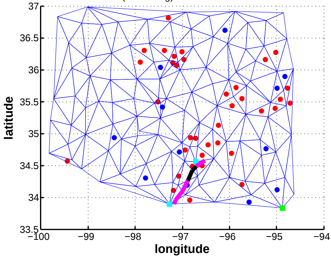
Mesonet Cold Pool Div. (15min avg) and Cold Pool Scores 1900z 4/25/2011
