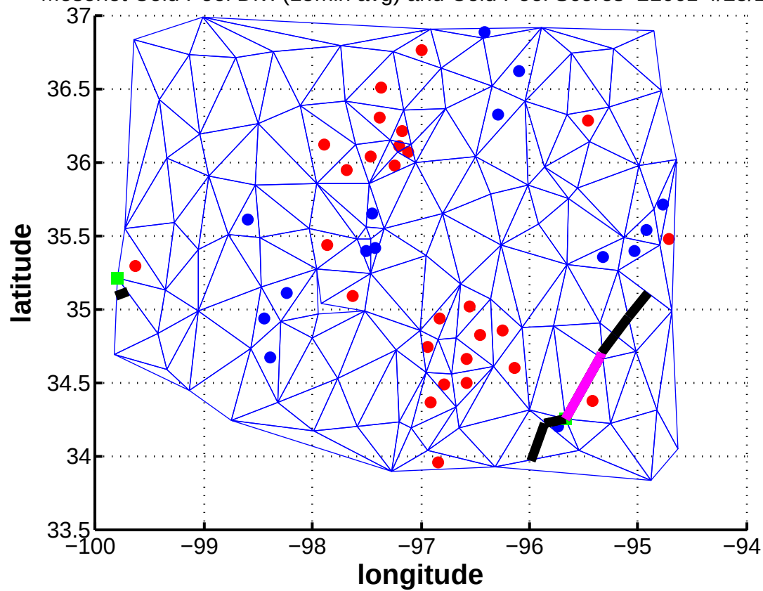
Mesonet Cold Pool Div. (15min avg) and Cold Pool Scores 2100z 4/25/2011
