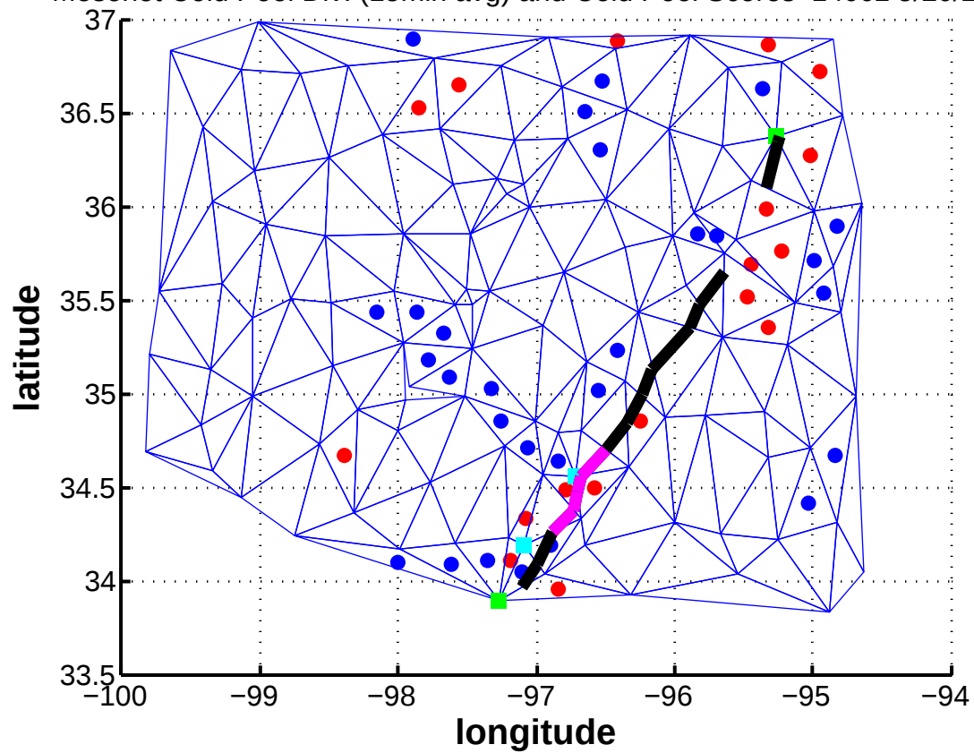
Mesonet Cold Pool Div. (15min avg) and Cold Pool Scores 1400z 5/20/2011
