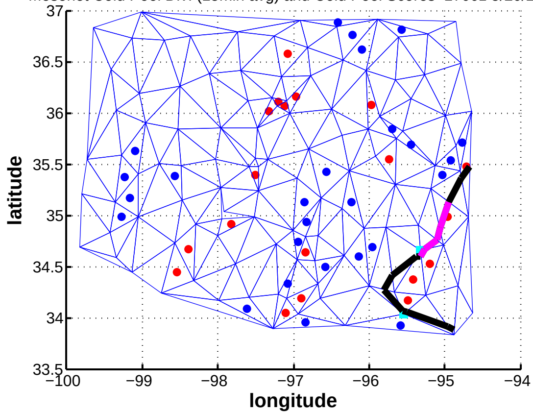
Mesonet Cold Pool Div. (15min avg) and Cold Pool Scores 1700z 5/20/2011
