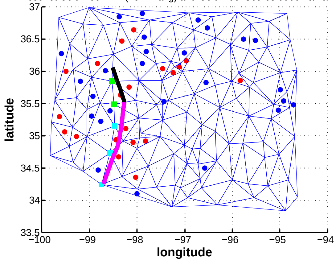
Mesonet Cold Pool Div. (15min avg) and Cold Pool Scores 0900z 5/20/2011
