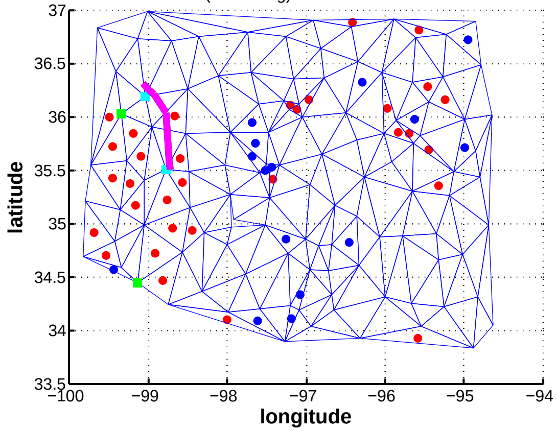
Mesonet Cold Pool Div. (15min avg) and Cold Pool Scores 2000z 5/24/2011
