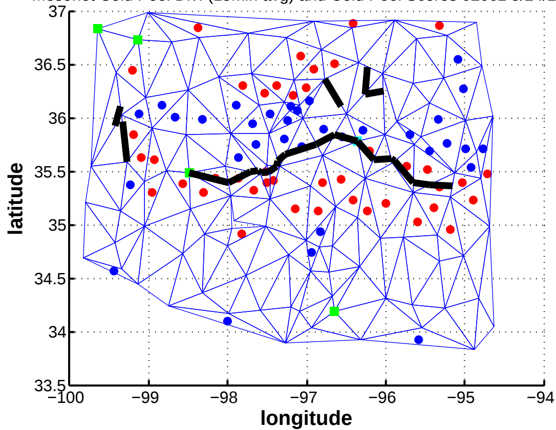
Mesonet Cold Pool Div. (15min avg) and Cold Pool Scores 0200z 5/24/2011
