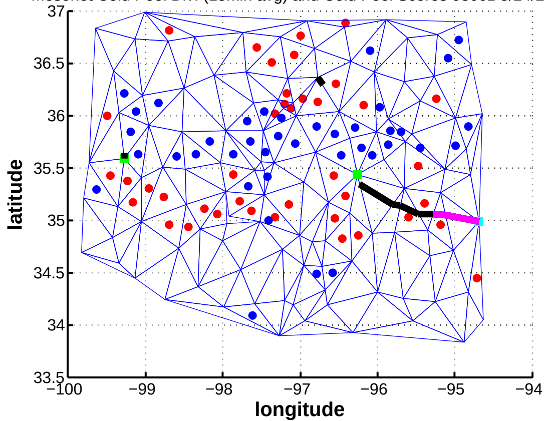
Mesonet Cold Pool Div. (15min avg) and Cold Pool Scores 0300z 5/24/2011
