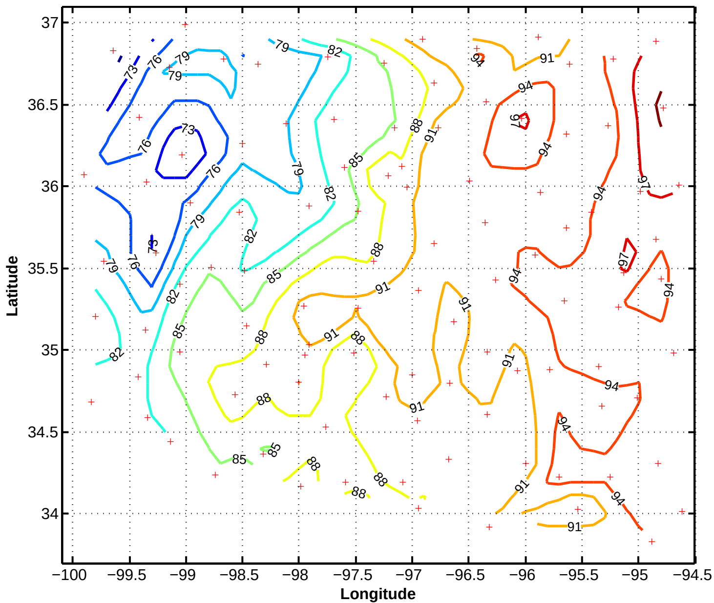
6/11/97 1230z Mesonet Pressure in .1mb above 970mb
