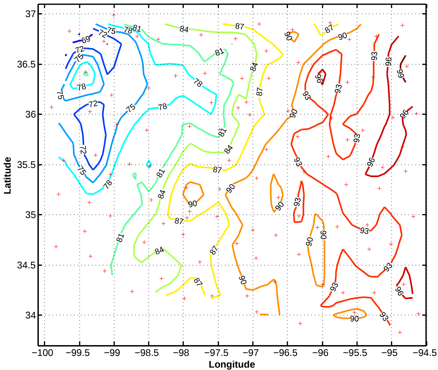
6/11/97 1300z Mesonet Pressure in .1mb above 970mb
