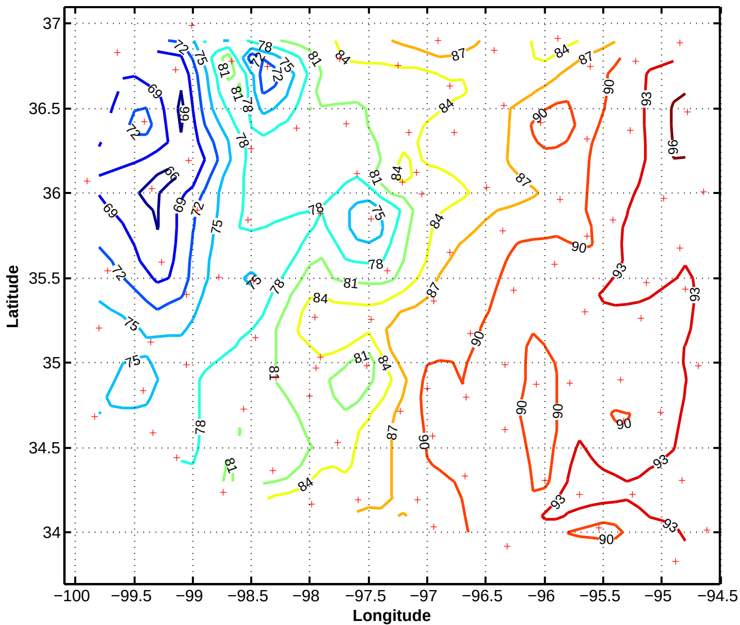
6/11/97 1330z Mesonet Pressure in .1mb above 970mb
