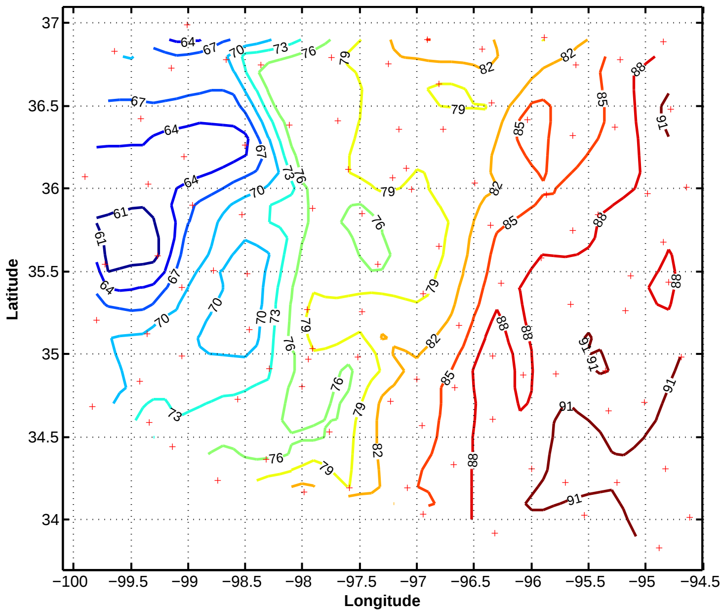
6/11/97 1430z Mesonet Pressure in .1mb above 970mb
