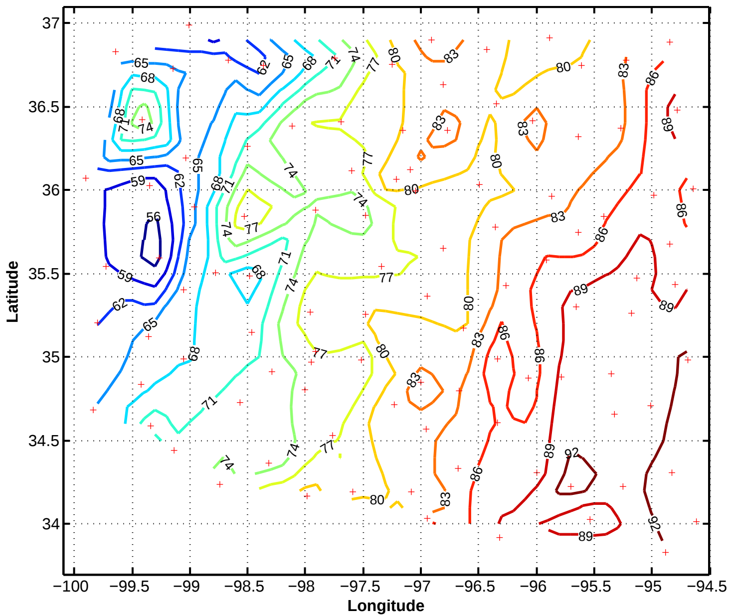
6/11/97 1500z Mesonet Pressure in .1mb above 970mb
