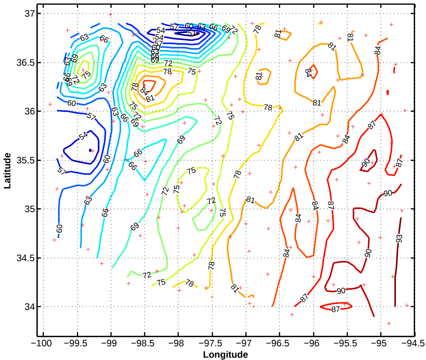
6/11/97 1530z Mesonet Pressure in .1mb above 970mb
