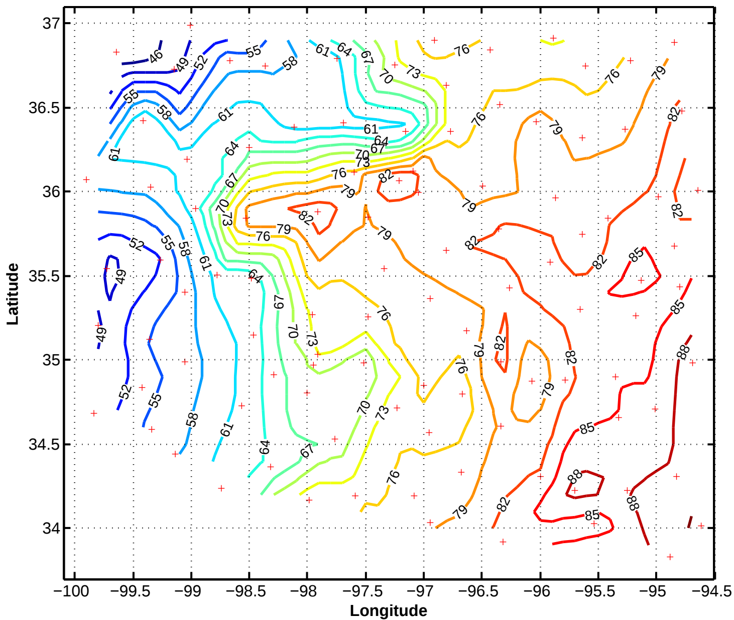
6/11/97 1700z Mesonet Pressure in .1mb above 970mb
