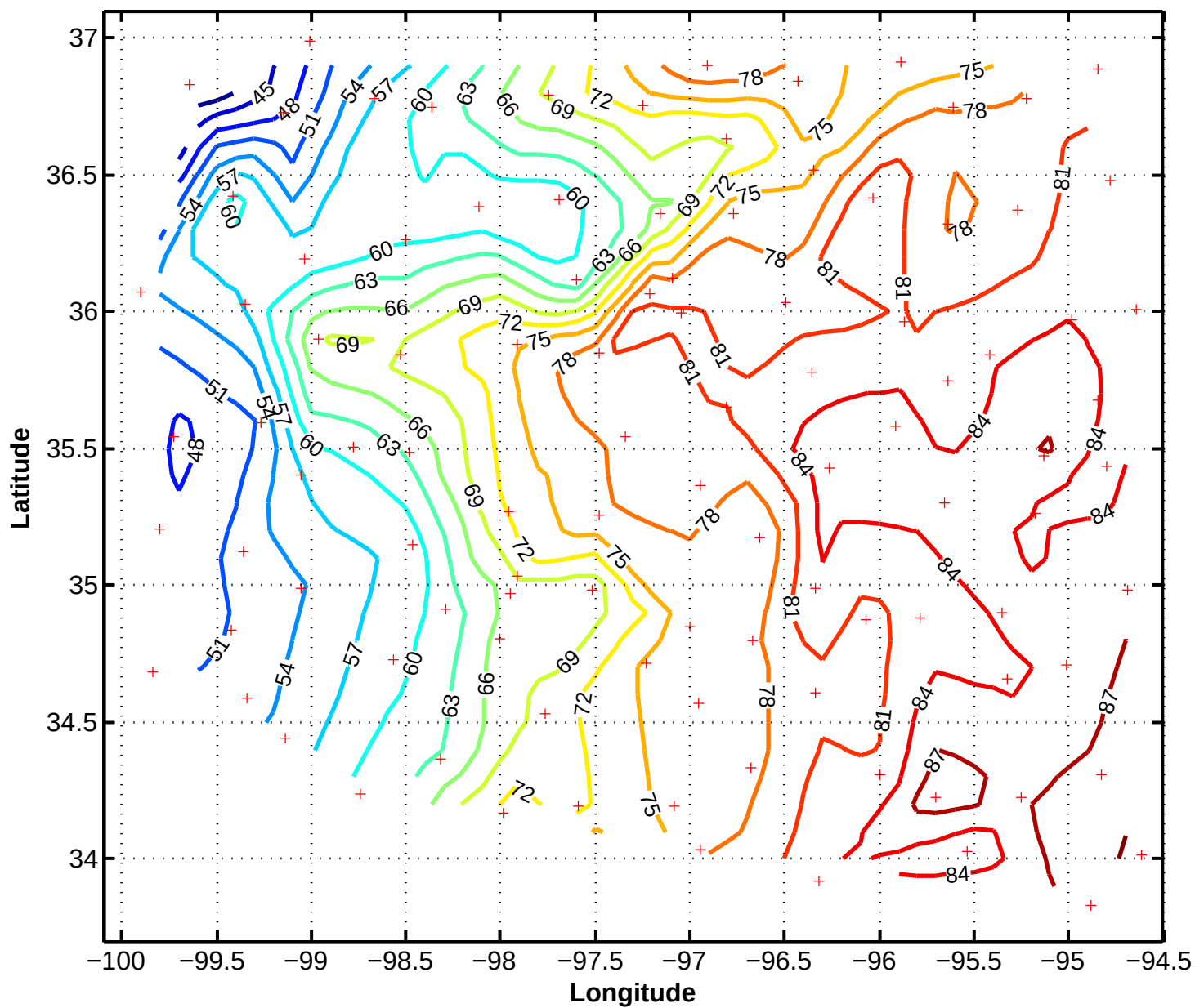
6/11/97 1730z Mesonet Pressure in .1mb above 970mb
