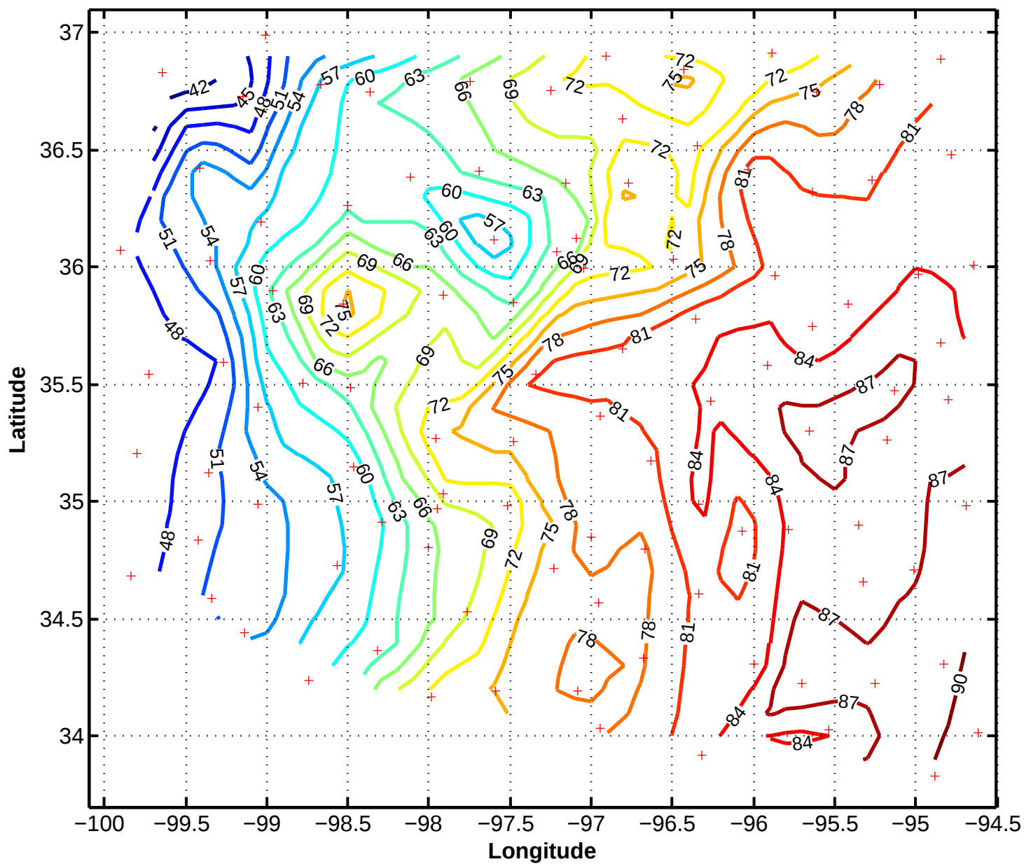
6/11/97 1800z Mesonet Pressure in .1mb above 970mb
