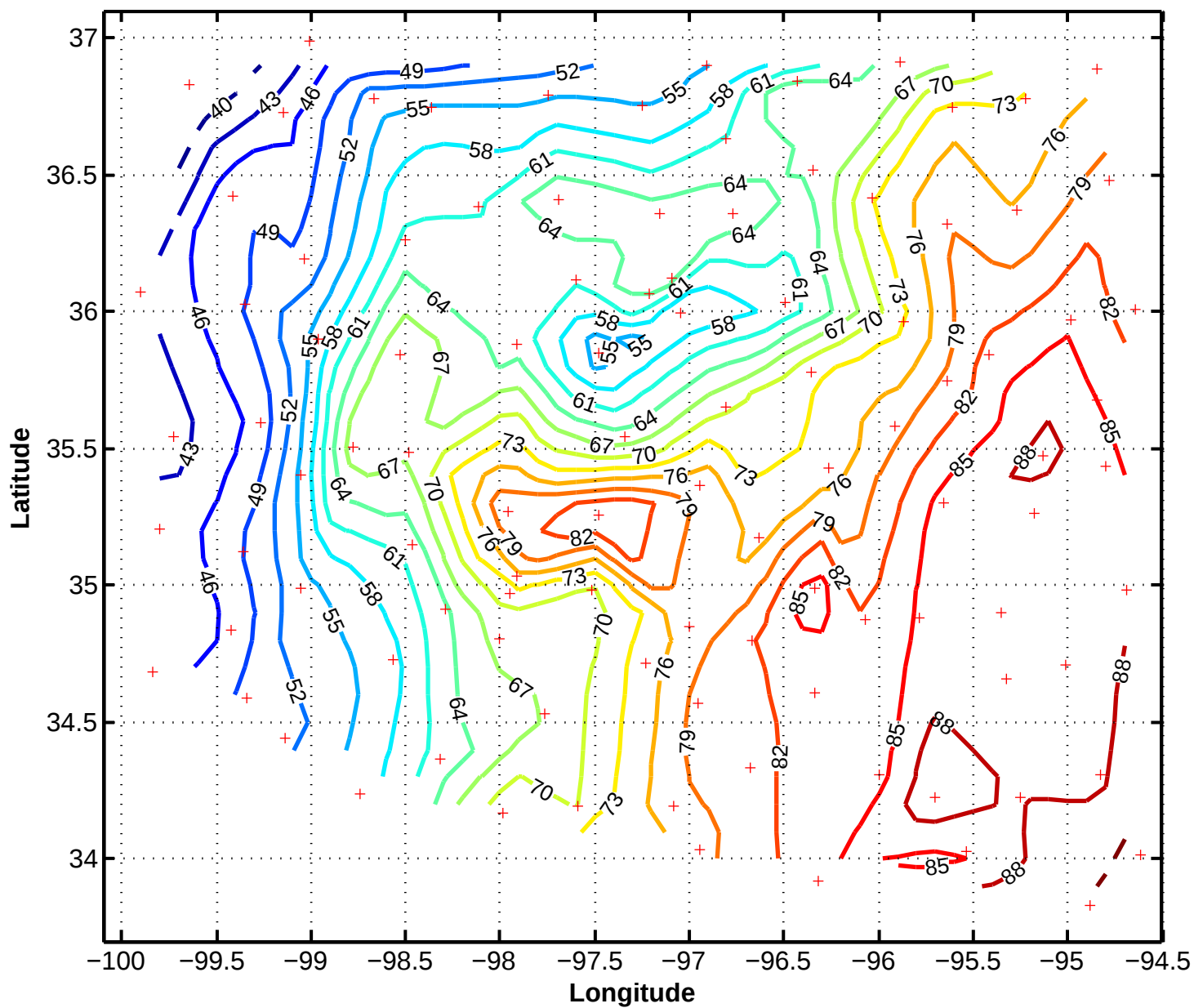
6/11/97 1900z Mesonet Pressure in .1mb above 970mb
