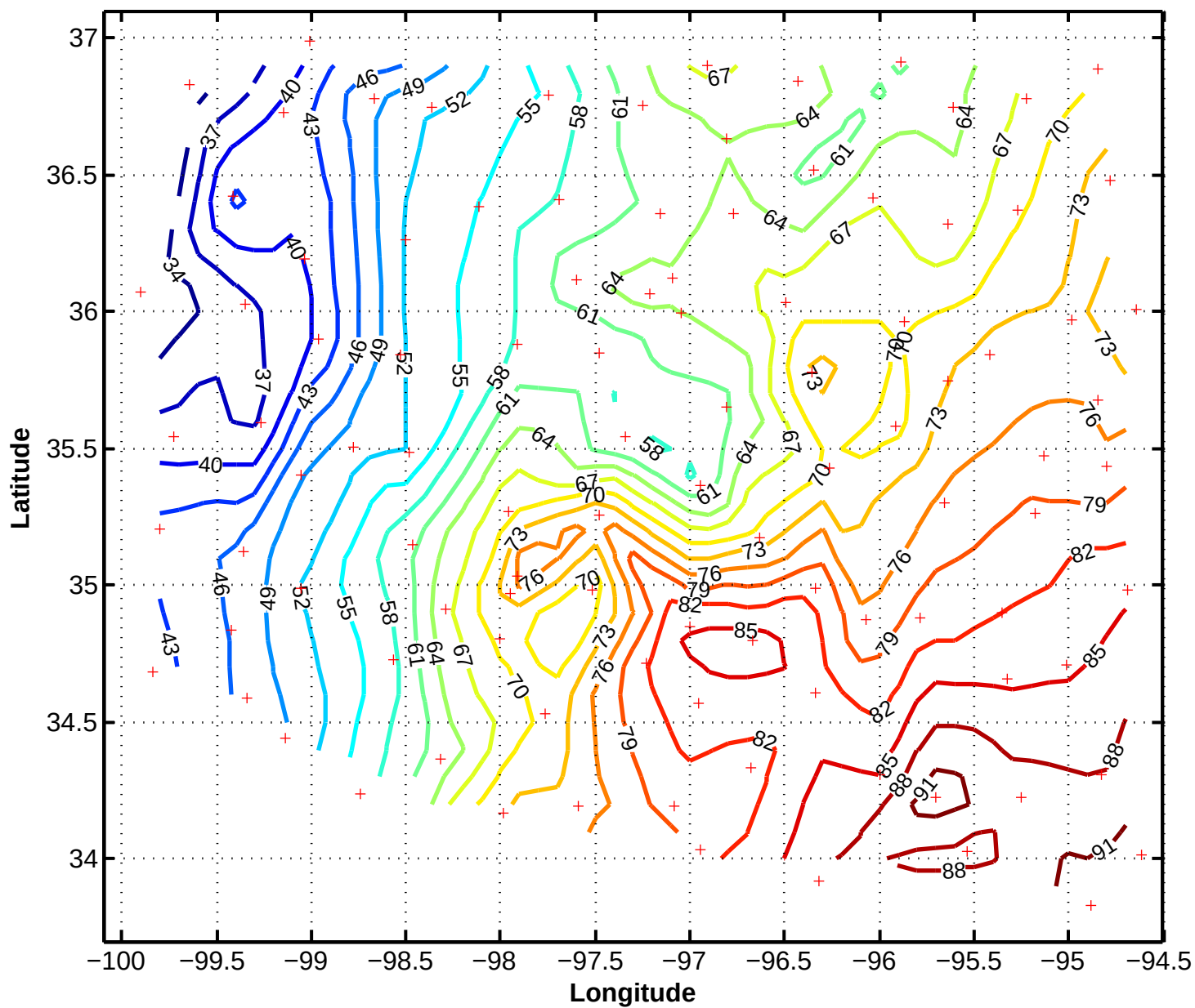
6/11/97 2030z Mesonet Pressure in .1mb above 970mb
