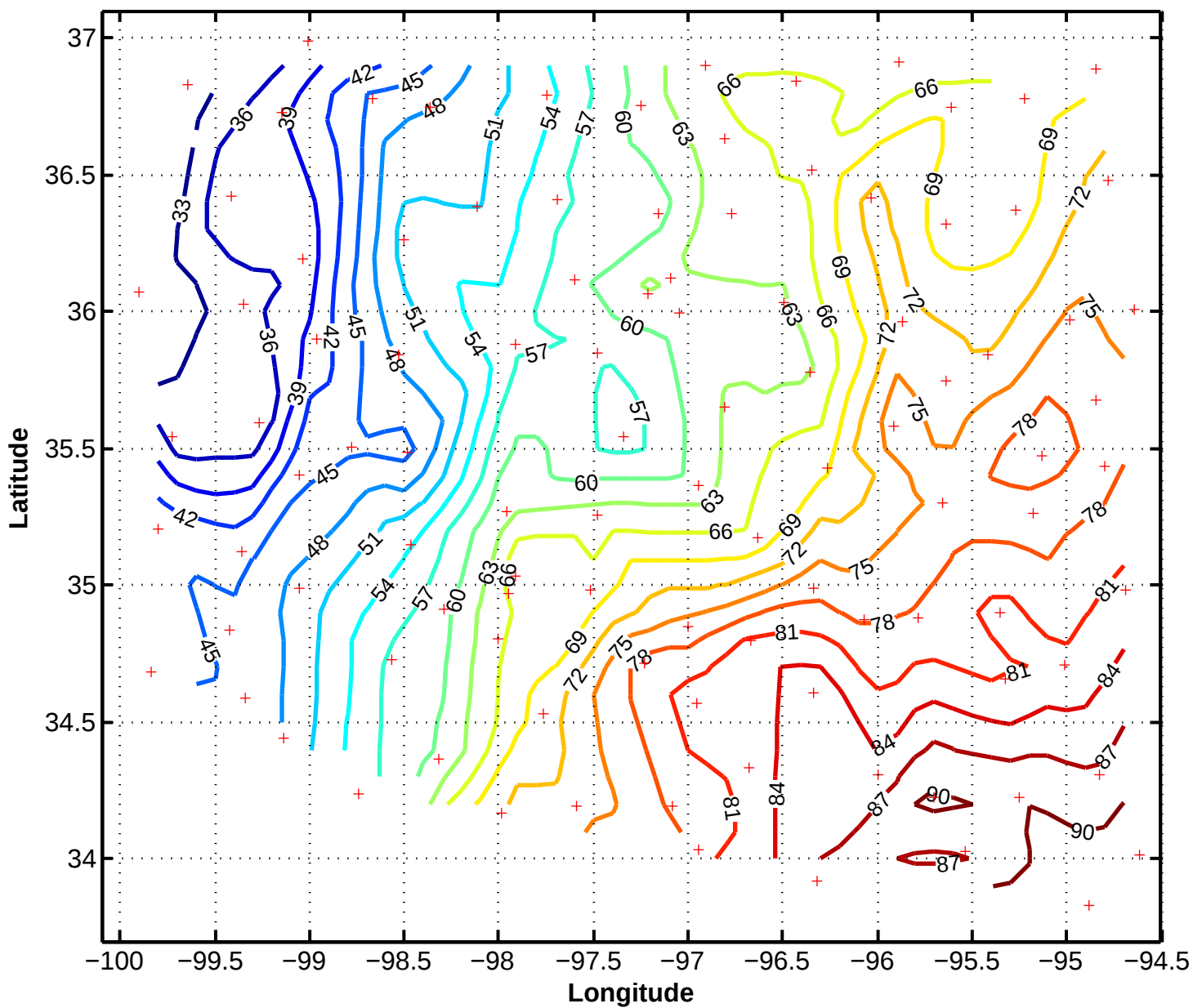
6/11/97 2100z Mesonet Pressure in .1mb above 970mb
