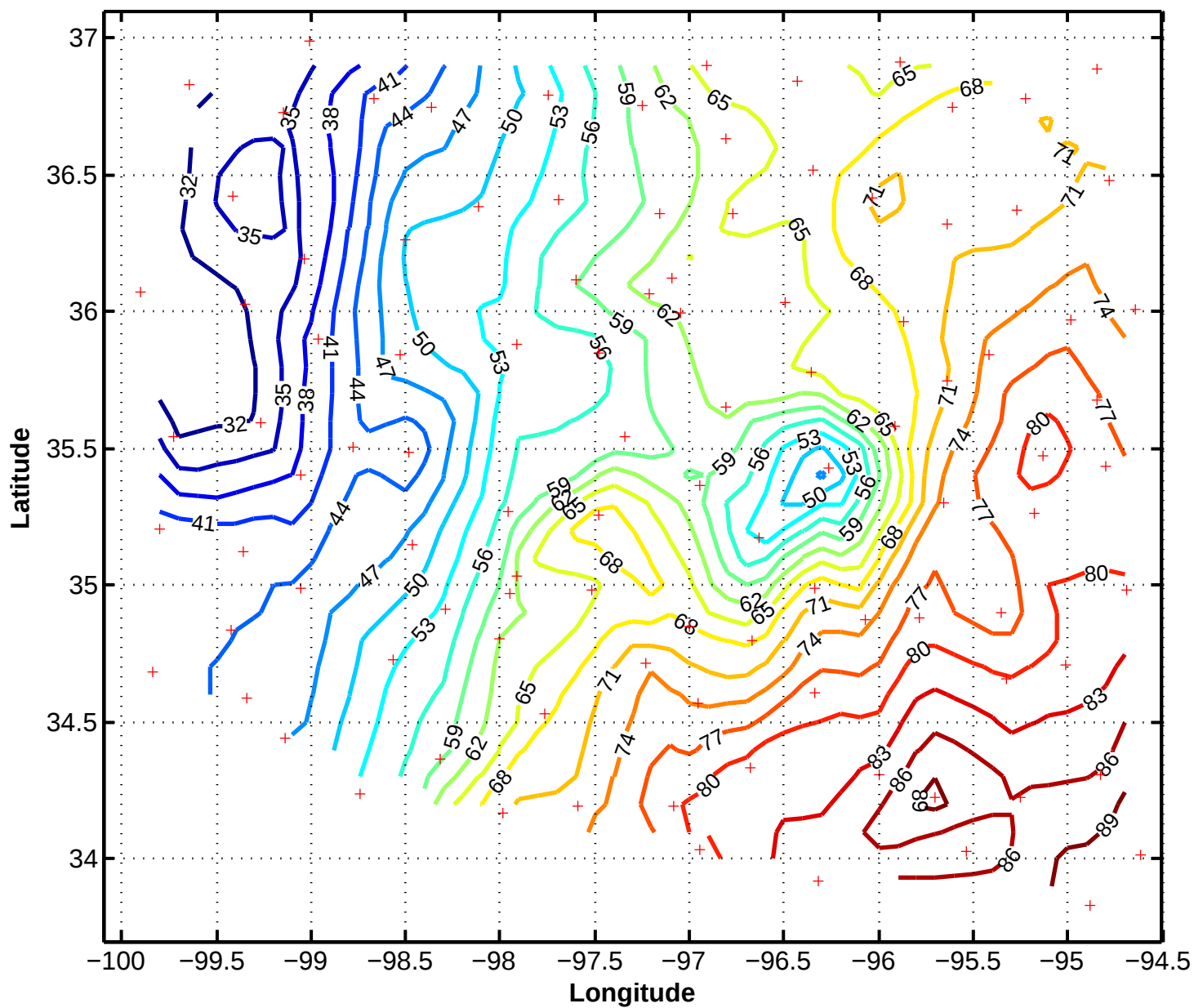
6/11/97 2130z Mesonet Pressure in .1mb above 970mb
