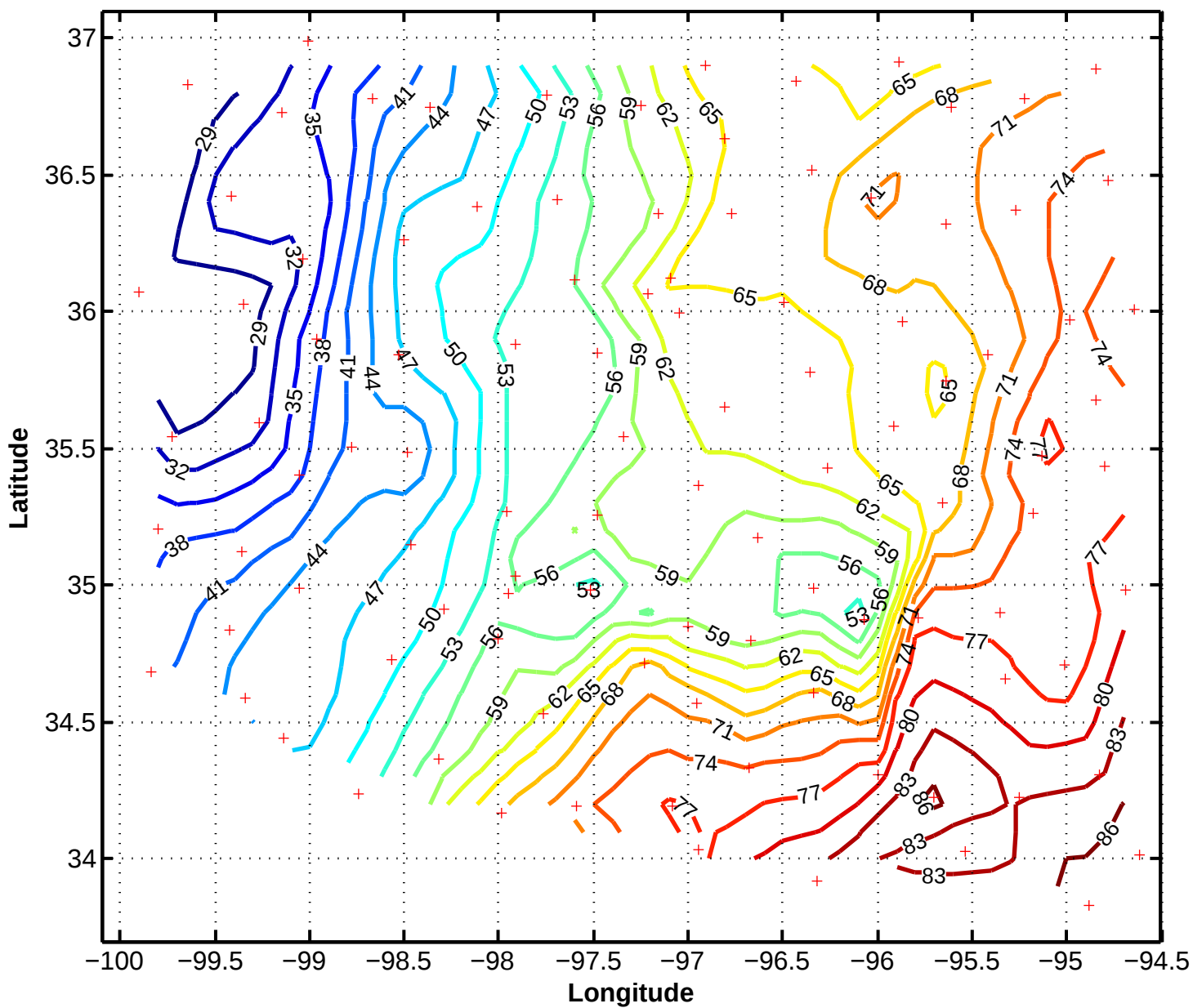
6/11/97 2200z Mesonet Pressure in .1mb above 970mb
