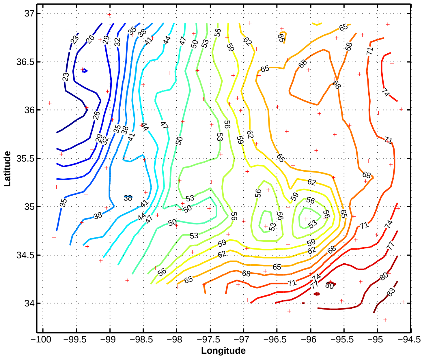
6/11/97 2230z Mesonet Pressure in .1mb above 970mb
