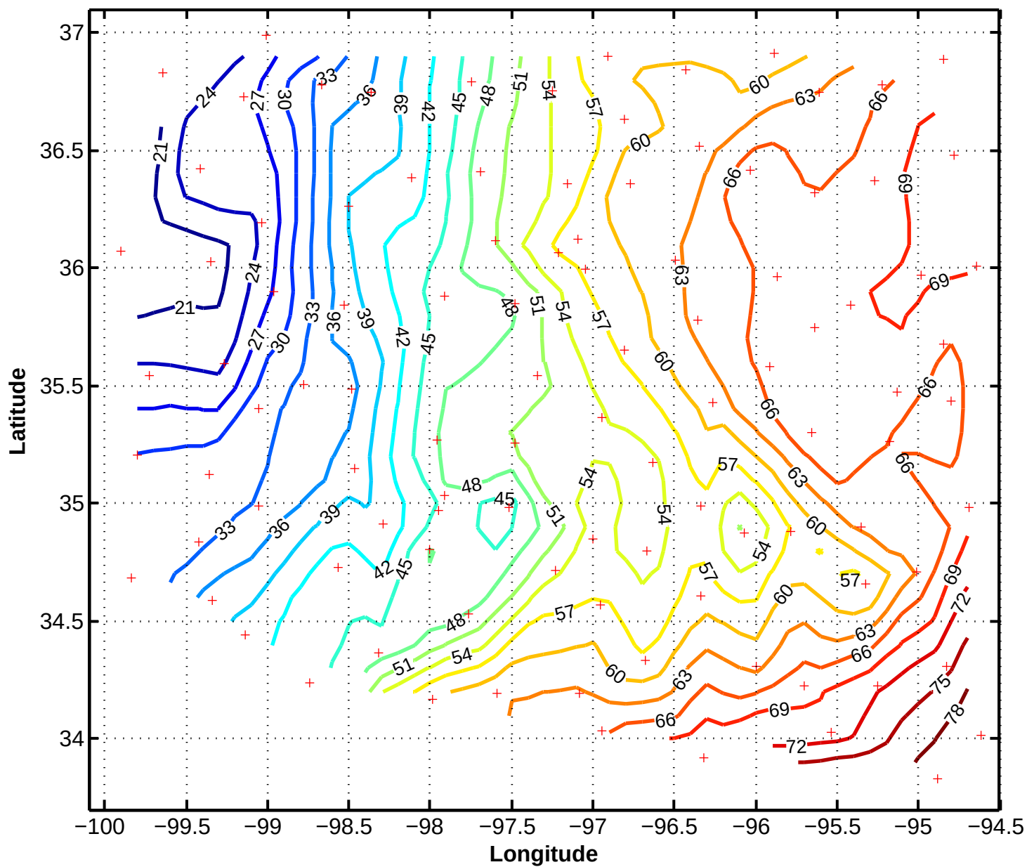
6/11/97 2300z Mesonet Pressure in .1mb above 970mb
