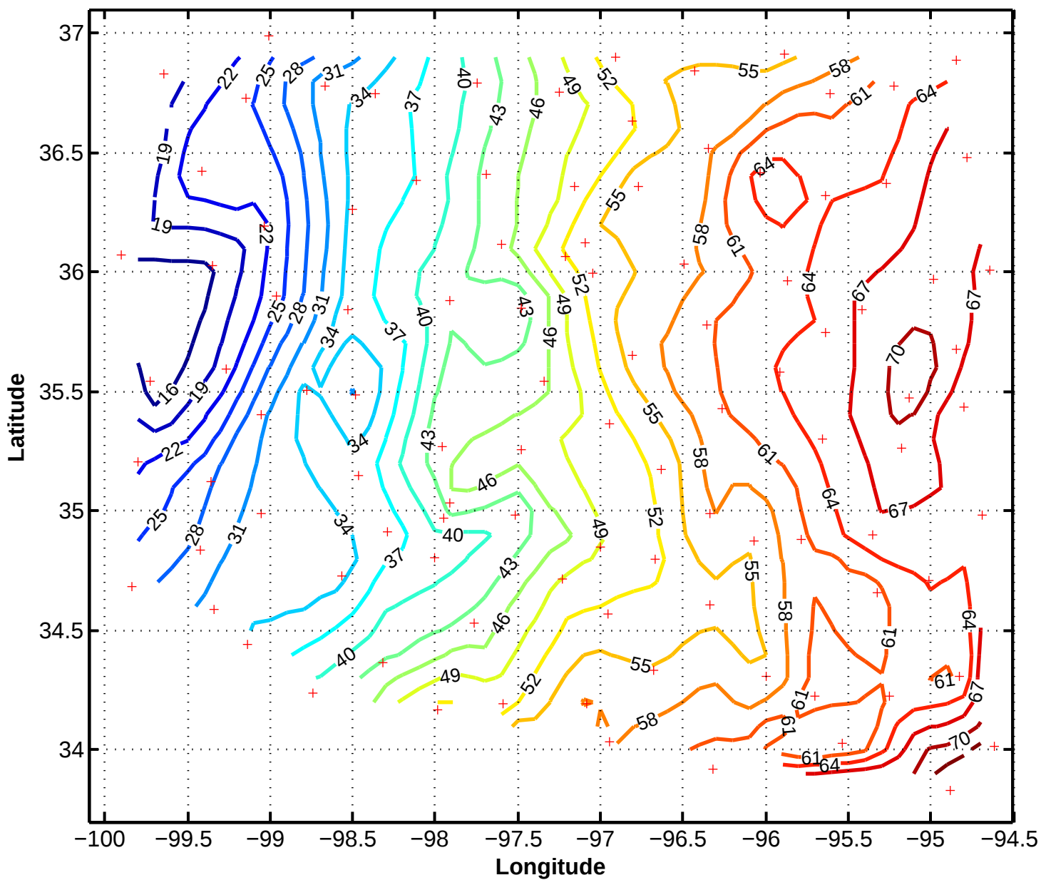
6/11/97 2330z Mesonet Pressure in .1mb above 970mb
